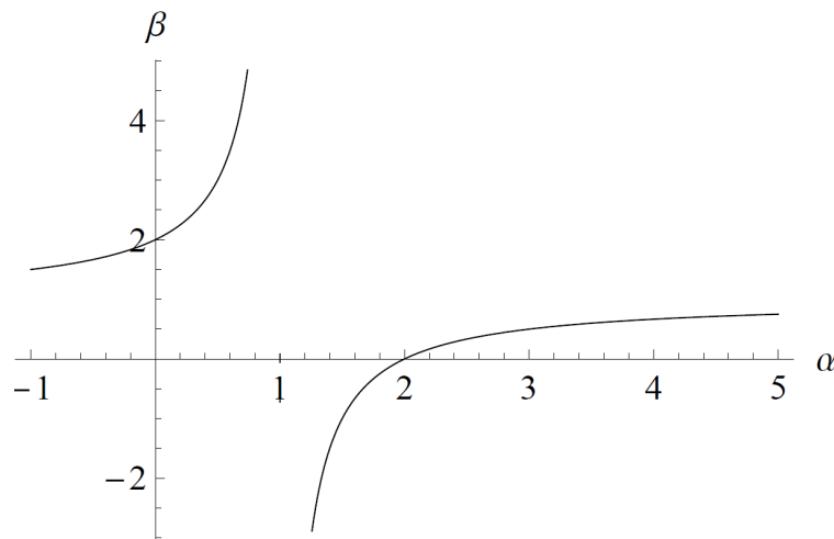
Figure 1 – Implied \beta for a given observation of \alpha , when \eta=2
